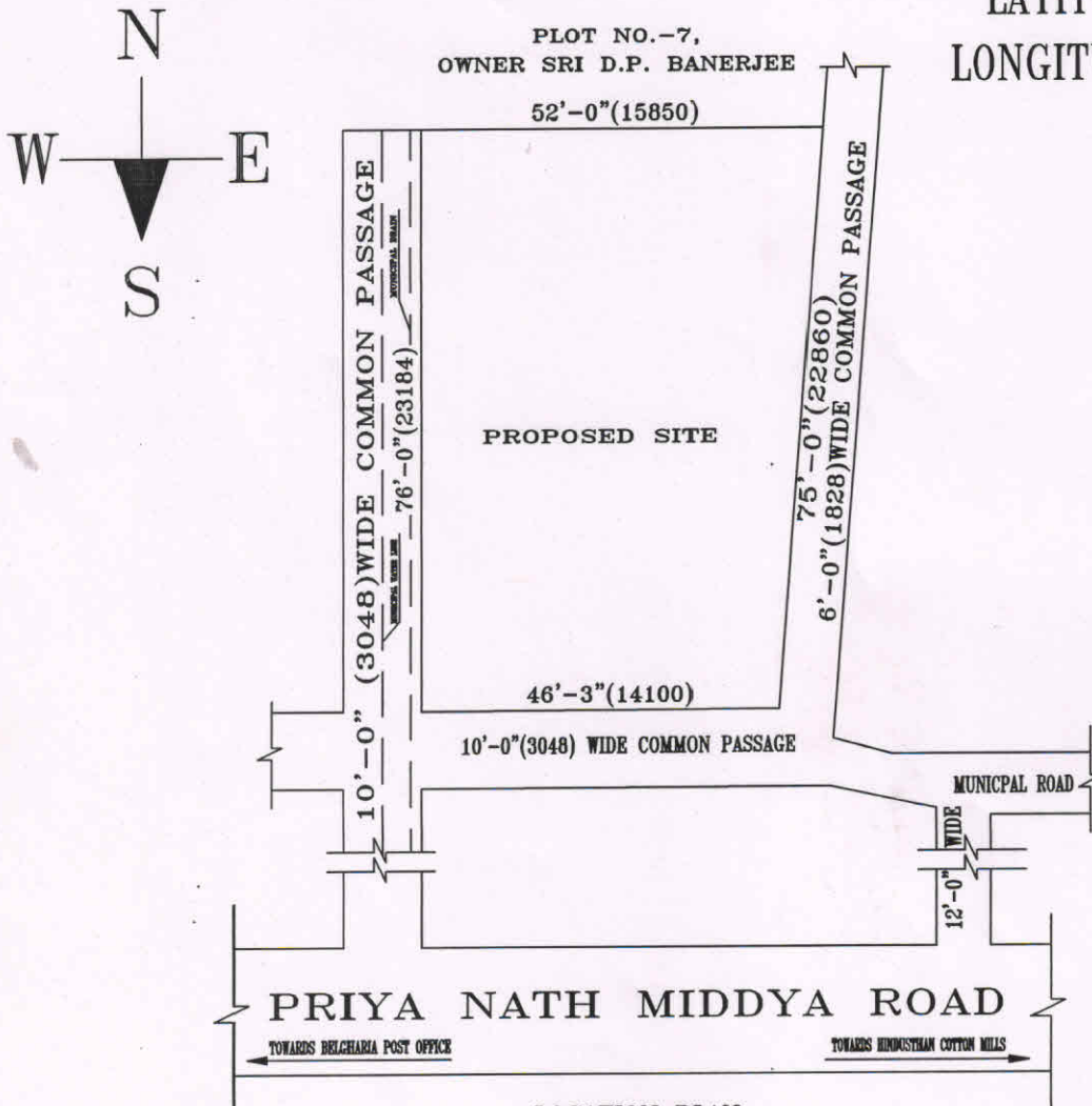
LOCATION PLAN SCALE=1:400
